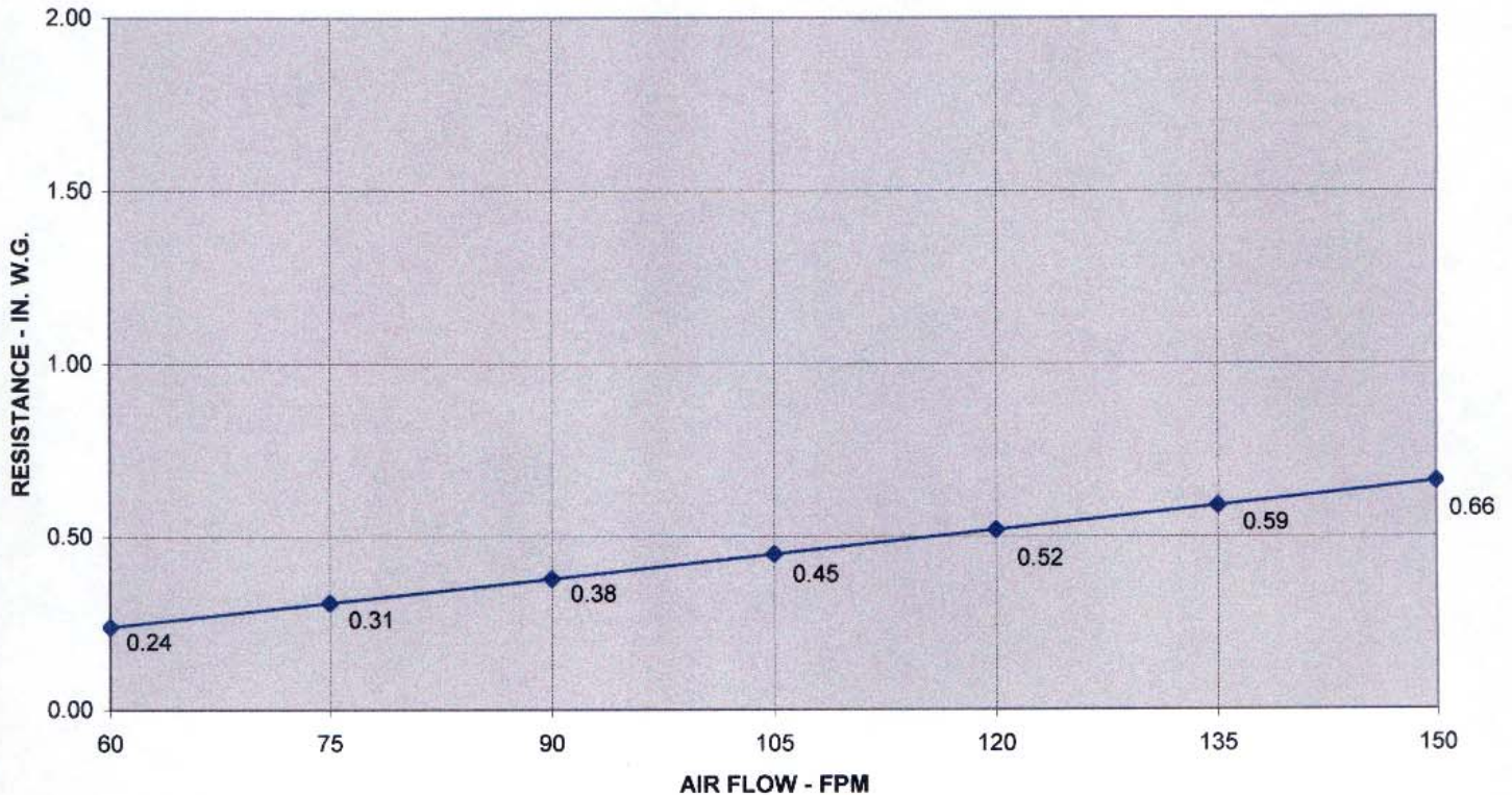
AIR FLOW VS RESISTANCE
